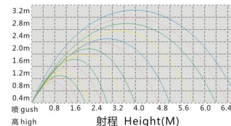
光亮泉跳泉设备射程曲线图 Light jump springs equipment range graphs springs
