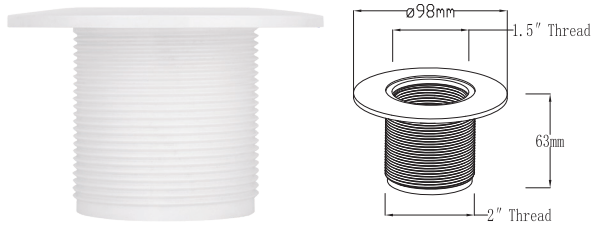
2"螺纹转接配件 / 2" Thread adapter fitting
